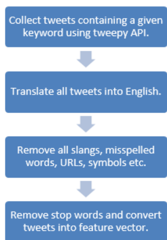
Fig. 2. Algorithm for preprocessing of data
